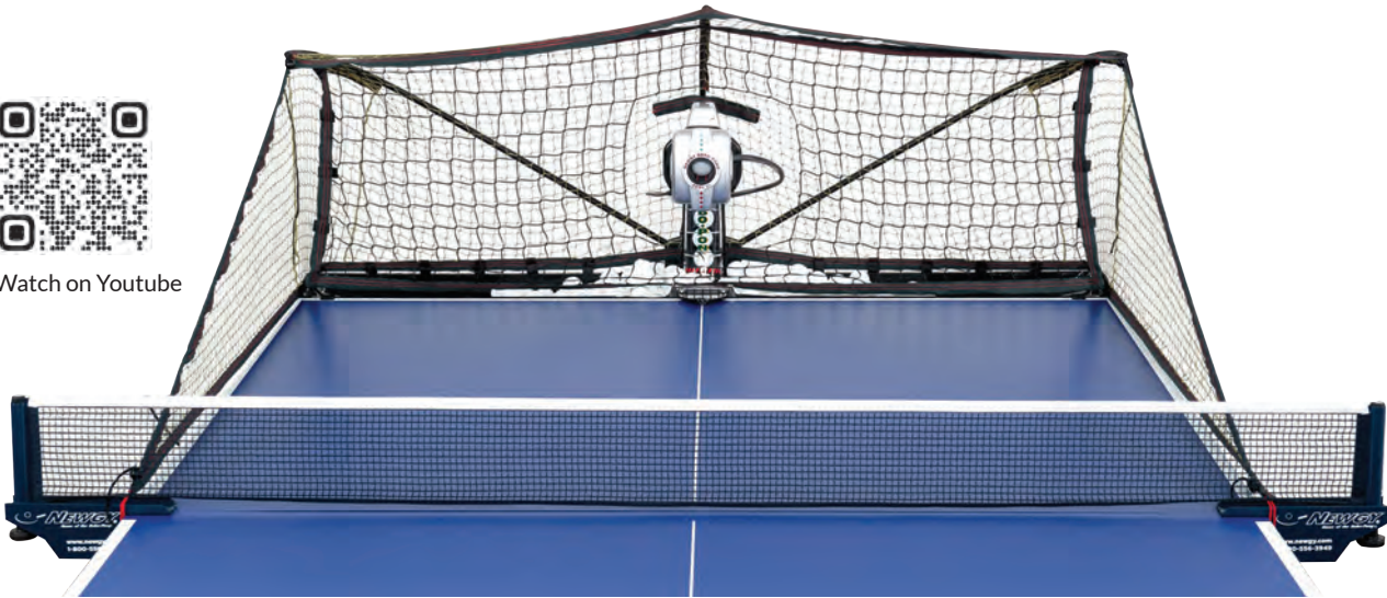
Robot functions through Bluetooth®, 2-Wheeled Ball Thrower (w/Oscillation)
